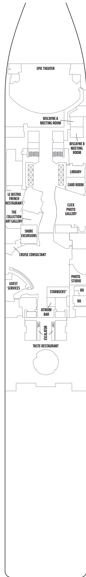
DECK 5
